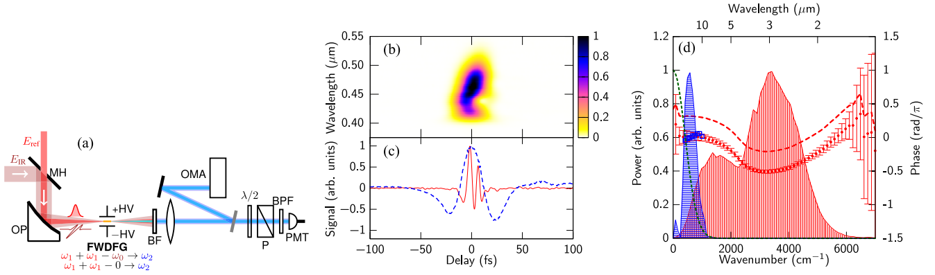
Fig. 6. (a) Schematic of the experiment for the waveform measurement, FROG-CEP. MH: aluminium-coated mirror with a hole ( \phi = 7 mm), OP: aluminium-coated off-axis parabolic mirror ( f = 150 mm), BF: blue filter (FGB37, Thorlabs), \lambda/2 : half wave plate, P: calcite polarizer, BPF: bandpass filter at 400 nm (10 nm FWHM), OMA: spectrometer for ultraviolet region (USB2000+, Ocean Optics). (b) The XFROG trace and (c) EOS signal (dashed curve) measured in the experiment. The solid curve shows the electric field reconstructed with the method described in the text. (d) The shaded (vertically hatched) and dashed curves are the spectral distribution and phase profile obtained with XFROG. The dots are the spectral phase after the offset correction. The offset of the spectral phase is corrected by using the phase information obtained with EOS. The error bars of the phase are estimated with the bootstrap method described in the text. The shaded (horizontally hatched) curve and open squares are the spectral distribution and spectral phase obtained from the Fourier transform of the EOS signal (dashed curve in (b)). The densely dashed curve shows the filtering function for the EOS signal, which is Fourier transform of |E_{ref}^2(t)|^2 . The FROG error was 0.3% on a 512 \times 512 grid.
