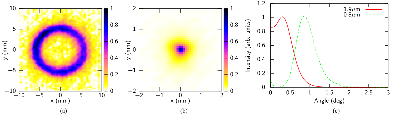
Fig. 4. (a) Experimental radial intensity distribution 250 mm after the generation point (on CM2 in Fig. 2(a)) of the IR pulses. (b) The intensity distribution at the focal point of the IR pulse focused with a concave mirror ( r = 2 m). (c) The intensity distribution of the IR signal as a function of the angle from the propagation axis. The solid and dotted curves show the IR intensities with 1.9 \mu\text{m} and 0.8 \mu\text{m} pump wavelength, respectively.
